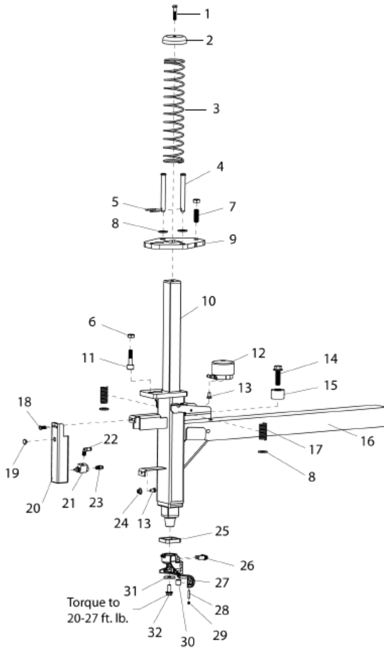
Steel DuckHead® Mount/Demount Tool
