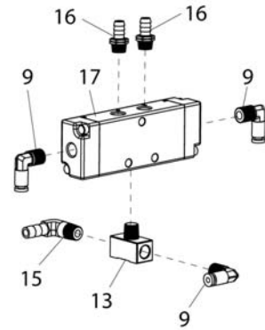
Pilot Valve Assembly 85610045
